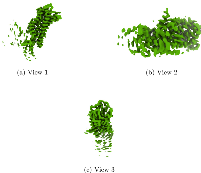
Figure 4: Isosurface at threshold=0.014000. Views generated by ChimeraX at a the following X, Y, Z angles: View 1 (0, -90, -90), View 2 (-90, 0, -90), View 3 (0, 0, 0).
