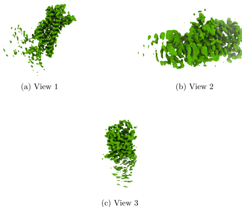
Figure 4: Isosurface at threshold=0.014100. Views generated by ChimeraX at a the following X, Y, Z angles: View 1 (0, -90, -90), View 2 (-90, 0, -90), View 3 (0, 0, 0).
