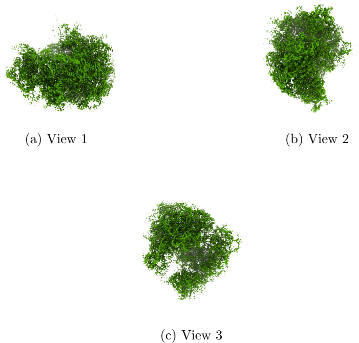
Figure 4: Isosurface at threshold=0.184000. Views generated by ChimeraX at a the following X, Y, Z angles: View 1 (0, -90, -90), View 2 (-90, 0, -90), View 3 (0, 0, 0).
