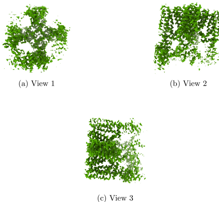
Figure 4: Isosurface at threshold=0.172000. Views generated by ChimeraX at a the following X, Y, Z angles: View 1 (0, -90, -90), View 2 (-90, 0, -90), View 3 (0, 0, 0).
