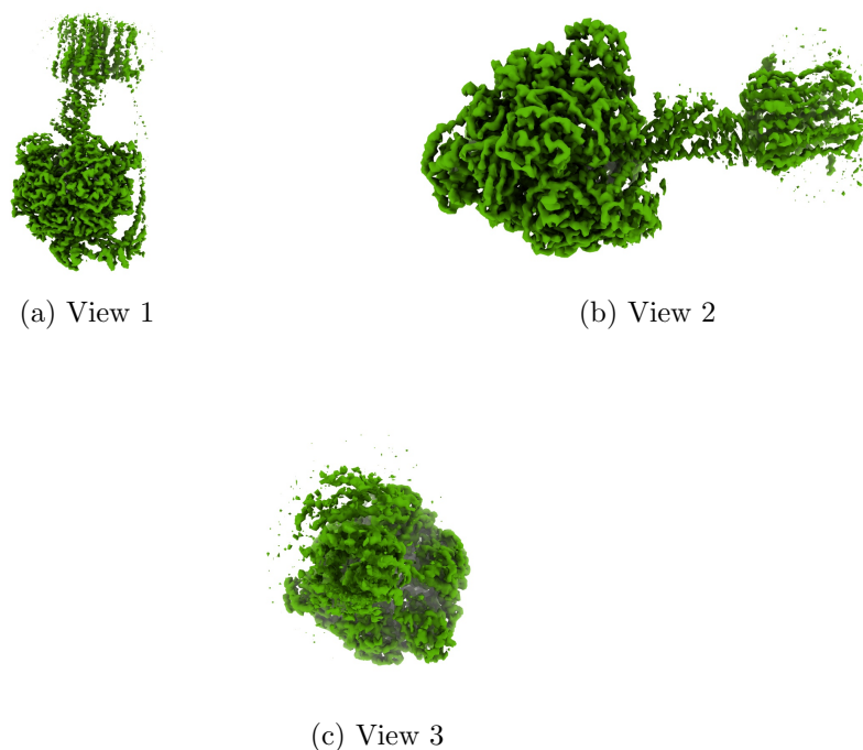
Figure 4: Isosurface at threshold=0.006310. Views generated by ChimeraX at a the following X, Y, Z angles: View 1 (0, -90, -90), View 2 (-90, 0, -90), View 3 (0, 0, 0).
