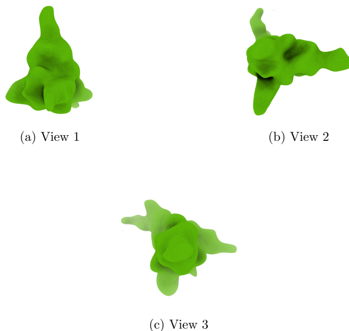
Figure 4: Isosurface at threshold=0.012500. Views generated by ChimeraX at a the following X, Y, Z angles: View 1 (0, -90, -90), View 2 (-90, 0, -90), View 3 (0, 0, 0).
