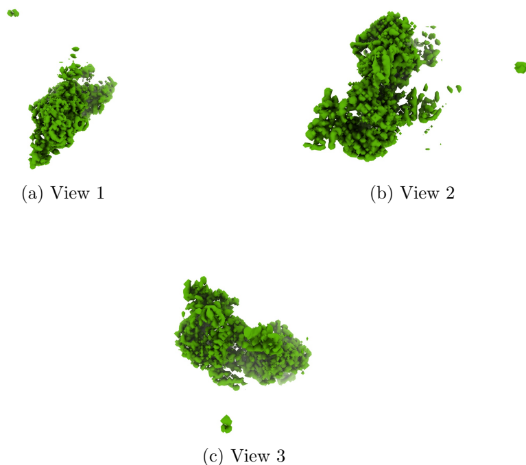
Figure 4: Isosurface at threshold=0.051800. Views generated by ChimeraX at a the following X, Y, Z angles: View 1 (0, -90, -90), View 2 (-90, 0, -90), View 3 (0, 0, 0).
