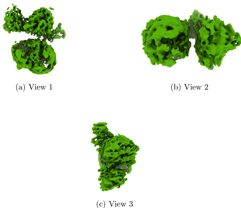
Figure 4: Isosurface at threshold=5.070000. Views generated by ChimeraX at a the following X, Y, Z angles: View 1 (0, -90, -90), View 2 (-90, 0, -90), View 3 (0, 0, 0).
