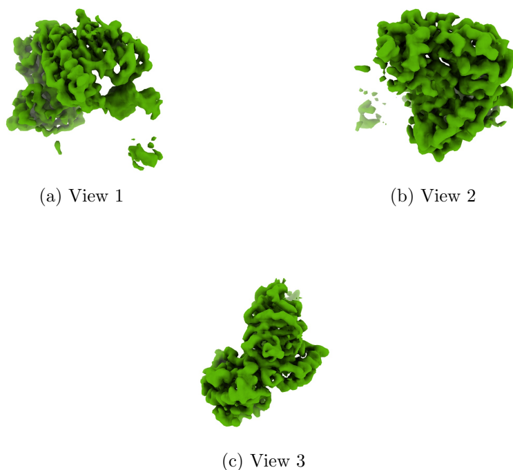
Figure 4: Isosurface at threshold=0.198000. Views generated by ChimeraX at a the following X, Y, Z angles: View 1 (0, -90, -90), View 2 (-90, 0, -90), View 3 (0, 0, 0).
