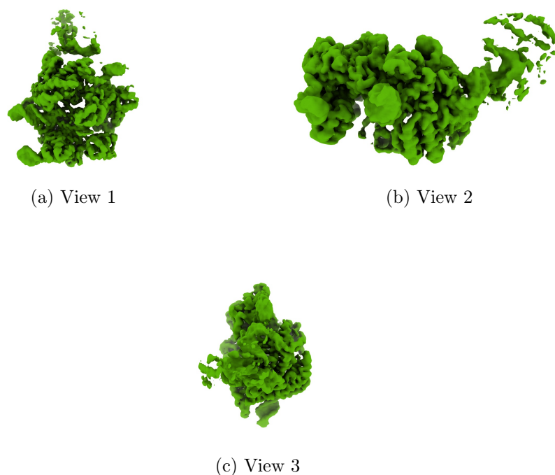
Figure 4: Isosurface at threshold=0.393000. Views generated by ChimeraX at a the following X, Y, Z angles: View 1 (0, -90, -90), View 2 (-90, 0, -90), View 3 (0, 0, 0).
