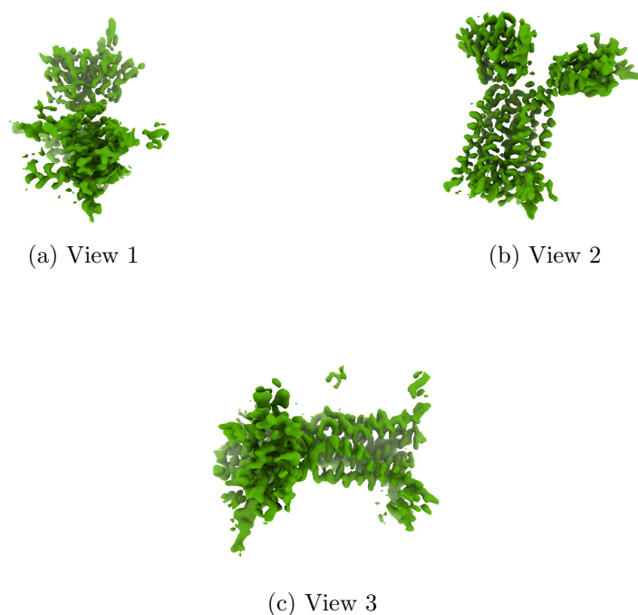
Figure 4: Isosurface at threshold=0.250000. Views generated by ChimeraX at a the following X, Y, Z angles: View 1 (0, -90, -90), View 2 (-90, 0, -90), View 3 (0, 0, 0).
