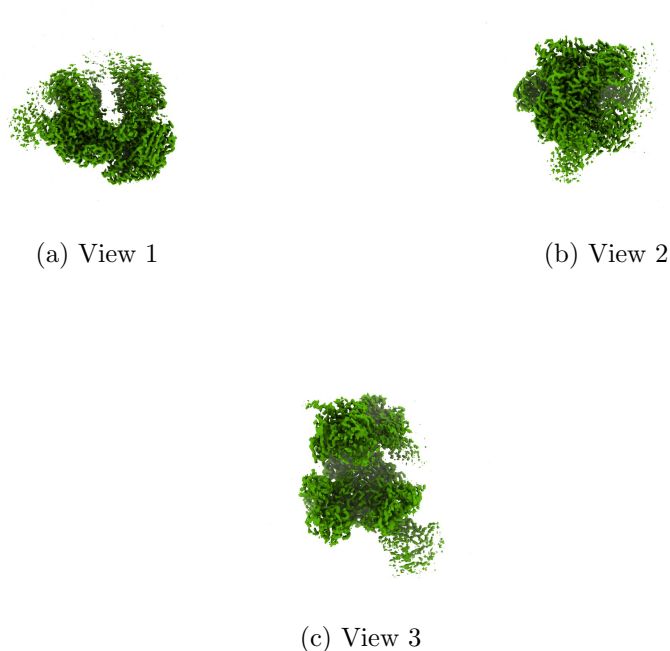
Figure 4: Isosurface at threshold=0.015600. Views generated by ChimeraX at a the following X, Y, Z angles: View 1 (0, -90, -90), View 2 (-90, 0, -90), View 3 (0, 0, 0).
