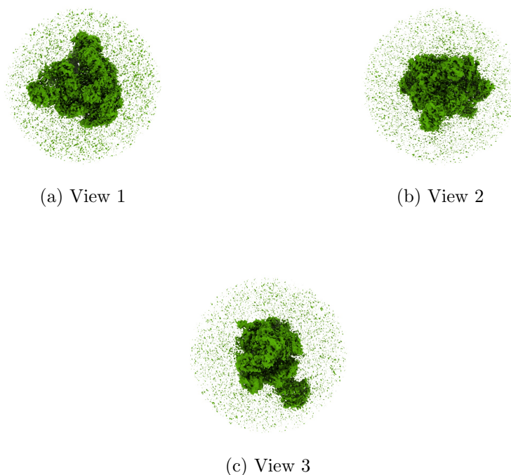
Figure 4: Isosurface at threshold=0.006090. Views generated by ChimeraX at a the following X, Y, Z angles: View 1 (0, -90, -90), View 2 (-90, 0, -90), View 3 (0, 0, 0).
