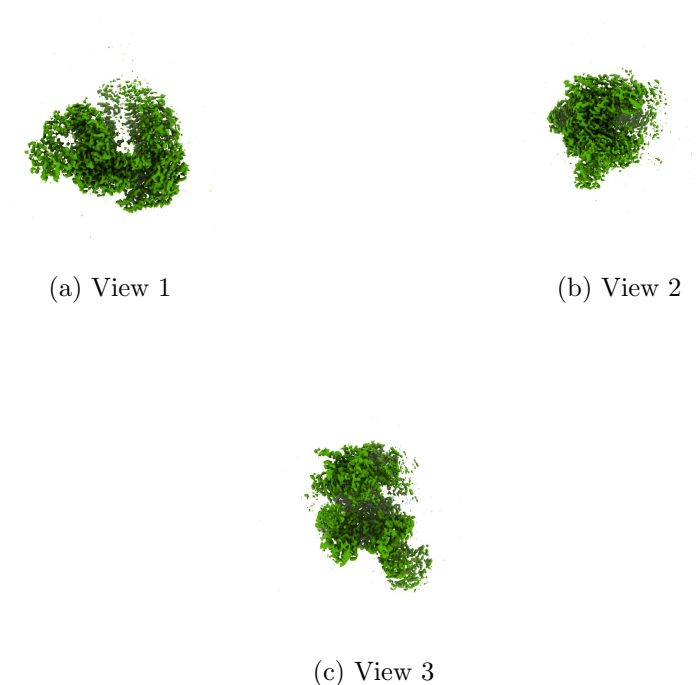
Figure 4: Isosurface at threshold=0.011600. Views generated by ChimeraX at a the following X, Y, Z angles: View 1 (0, -90, -90), View 2 (-90, 0, -90), View 3 (0, 0, 0).
