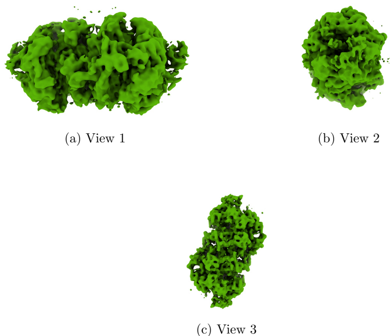
Figure 4: Isosurface at threshold=0.680000. Views generated by ChimeraX at a the following X, Y, Z angles: View 1 (0, -90, -90), View 2 (-90, 0, -90), View 3 (0, 0, 0).
