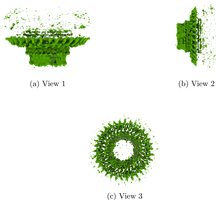
Figure 4: Isosurface at threshold=0.183000. Views generated by ChimeraX at a the following X, Y, Z angles: View 1 (0, -90, -90), View 2 (-90, 0, -90), View 3 (0, 0, 0).
