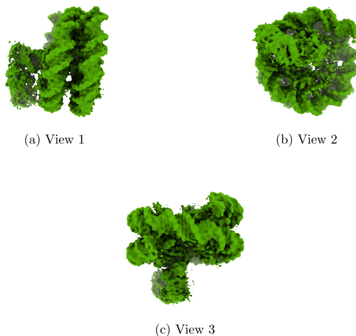
Figure 4: Isosurface at threshold=0.007000. Views generated by ChimeraX at a the following X, Y, Z angles: View 1 (0, -90, -90), View 2 (-90, 0, -90), View 3 (0, 0, 0).
