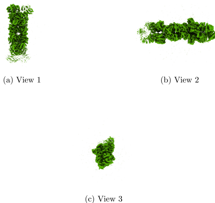
Figure 4: Isosurface at threshold=0.220000. Views generated by ChimeraX at a the following X, Y, Z angles: View 1 (0, -90, -90), View 2 (-90, 0, -90), View 3 (0, 0, 0).
