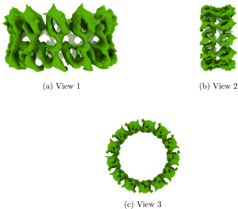
Figure 4: Isosurface at threshold=0.038500. Views generated by ChimeraX at a the following X, Y, Z angles: View 1 (0, -90, -90), View 2 (-90, 0, -90), View 3 (0, 0, 0).
