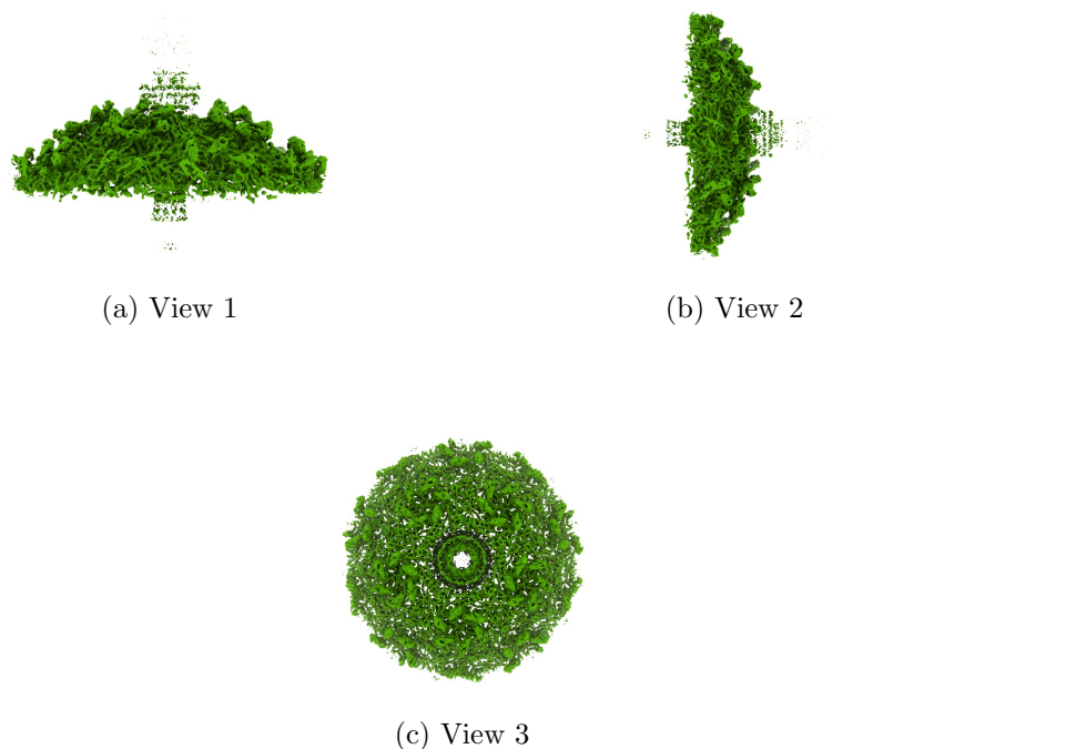
Figure 4: Isosurface at threshold=0.350000. Views generated by ChimeraX at a the following X, Y, Z angles: View 1 (0, -90, -90), View 2 (-90, 0, -90), View 3 (0, 0, 0).
