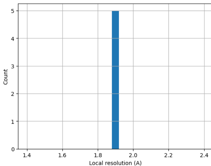
Figure 25: Histogram of the local resolution according to Resmap.
