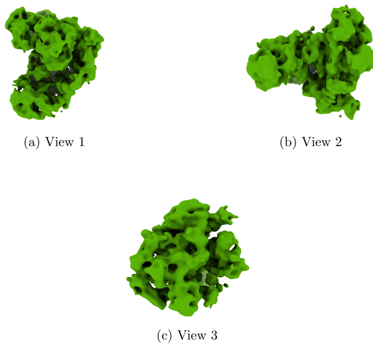
Figure 4: Isosurface at threshold=36.000000. Views generated by ChimeraX at a the following X, Y, Z angles: View 1 (0, -90, -90), View 2 (-90, 0, -90), View 3 (0, 0, 0).
