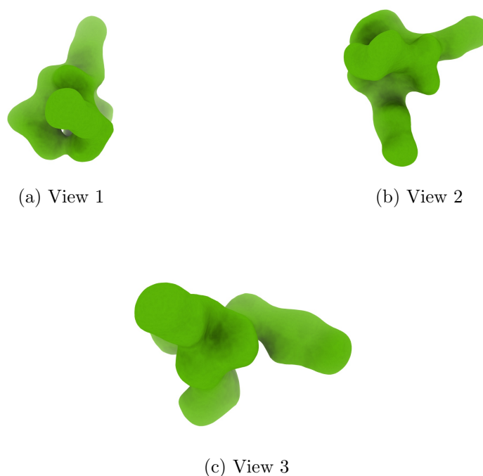
Figure 4: Isosurface at threshold=0.025000. Views generated by ChimeraX at a the following X, Y, Z angles: View 1 (0, -90, -90), View 2 (-90, 0, -90), View 3 (0, 0, 0).
