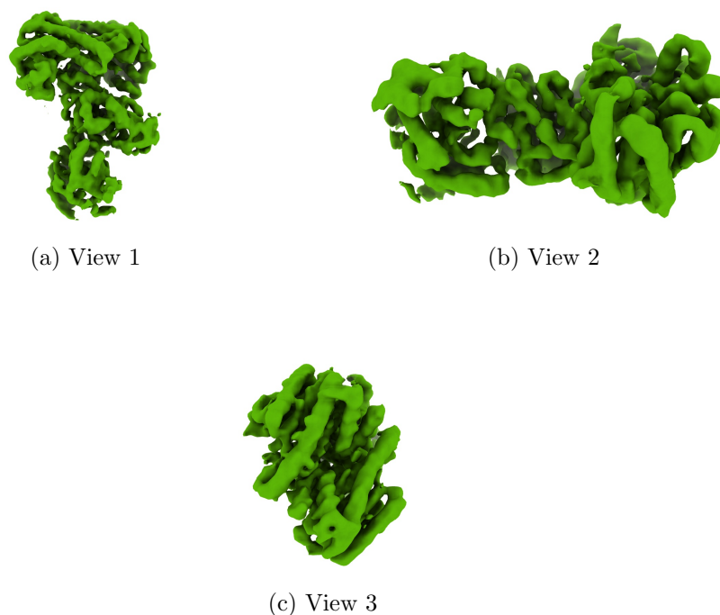
Figure 4: Isosurface at threshold=0.321000. Views generated by ChimeraX at a the following X, Y, Z angles: View 1 (0, -90, -90), View 2 (-90, 0, -90), View 3 (0, 0, 0).
