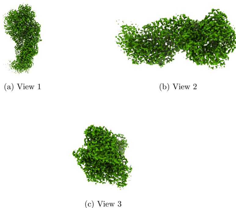
Figure 4: Isosurface at threshold=0.931000. Views generated by ChimeraX at a the following X, Y, Z angles: View 1 (0, -90, -90), View 2 (-90, 0, -90), View 3 (0, 0, 0).
