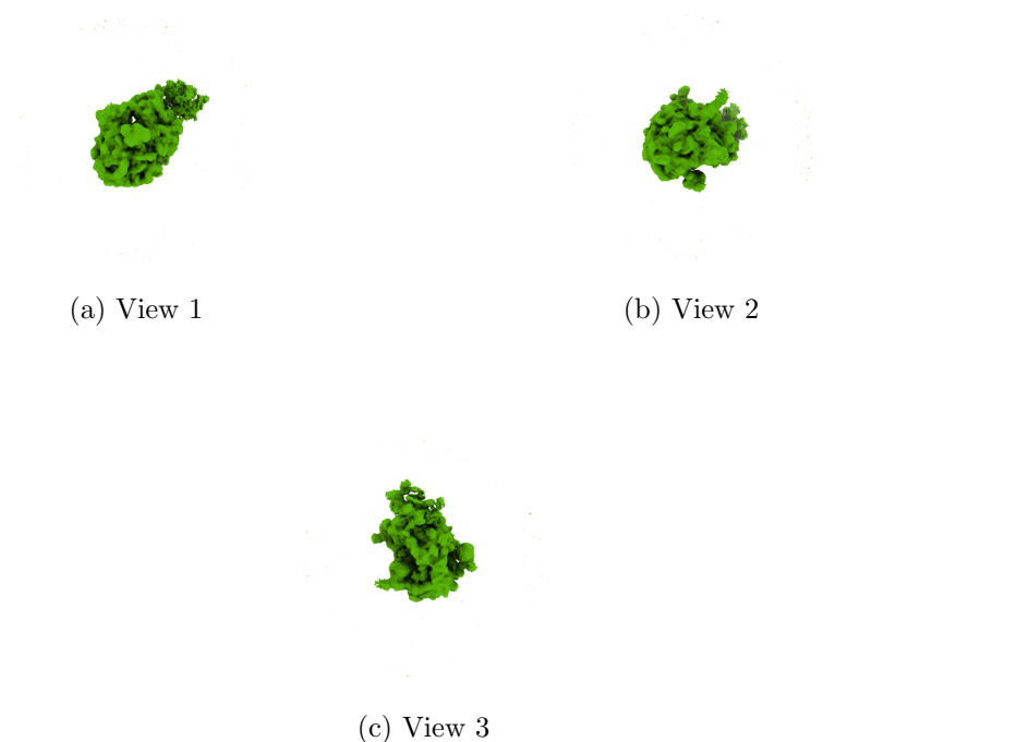
Figure 4: Isosurface at threshold=0.005000. Views generated by ChimeraX at a the following X, Y, Z angles: View 1 (0, -90, -90), View 2 (-90, 0, -90), View 3 (0, 0, 0).
