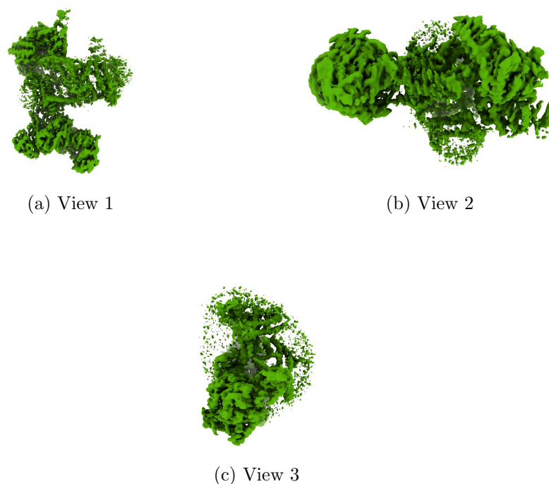
Figure 4: Isosurface at threshold=0.003420. Views generated by ChimeraX at a the following X, Y, Z angles: View 1 (0, -90, -90), View 2 (-90, 0, -90), View 3 (0, 0, 0).
