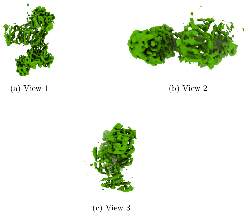
Figure 4: Isosurface at threshold=0.002700. Views generated by ChimeraX at a the following X, Y, Z angles: View 1 (0, -90, -90), View 2 (-90, 0, -90), View 3 (0, 0, 0).
