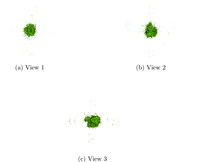
Figure 4: Isosurface at threshold=0.040000. Views generated by ChimeraX at a the following X, Y, Z angles: View 1 (0, -90, -90), View 2 (-90, 0, -90), View 3 (0, 0, 0).
