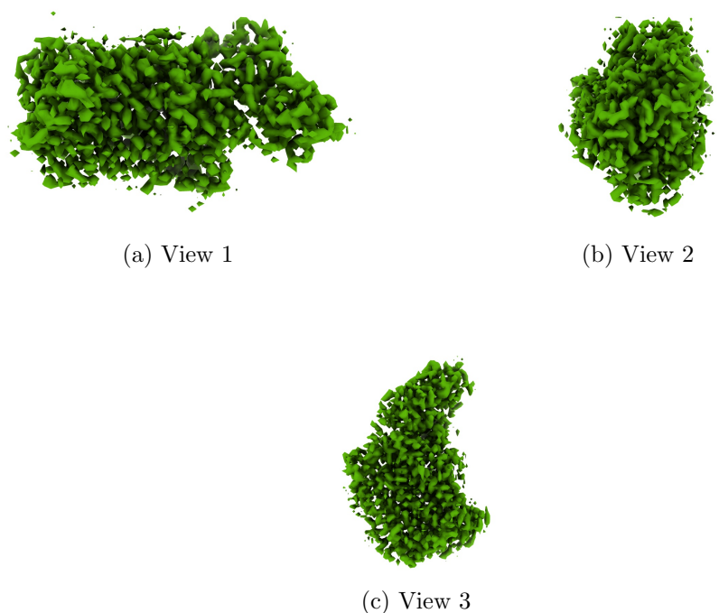
Figure 4: Isosurface at threshold=1.570000. Views generated by ChimeraX at a the following X, Y, Z angles: View 1 (0, -90, -90), View 2 (-90, 0, -90), View 3 (0, 0, 0).
