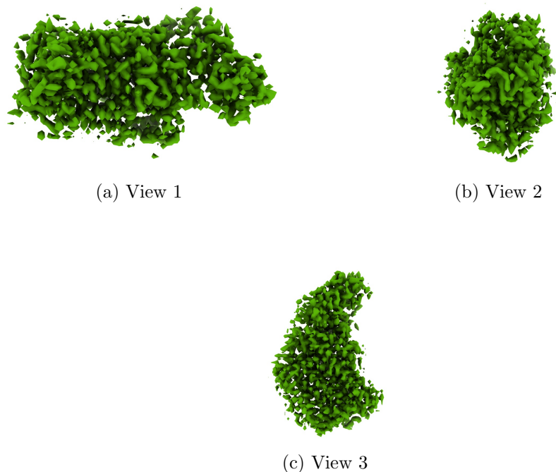
Figure 4: Isosurface at threshold=1.650000. Views generated by ChimeraX at a the following X, Y, Z angles: View 1 (0, -90, -90), View 2 (-90, 0, -90), View 3 (0, 0, 0).
