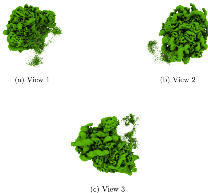
Figure 4: Isosurface at threshold=0.007130. Views generated by ChimeraX at a the following X, Y, Z angles: View 1 (0, -90, -90), View 2 (-90, 0, -90), View 3 (0, 0, 0).
