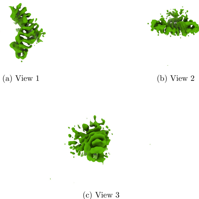
Figure 4: Isosurface at threshold=0.202000. Views generated by ChimeraX at a the following X, Y, Z angles: View 1 (0, -90, -90), View 2 (-90, 0, -90), View 3 (0, 0, 0).
