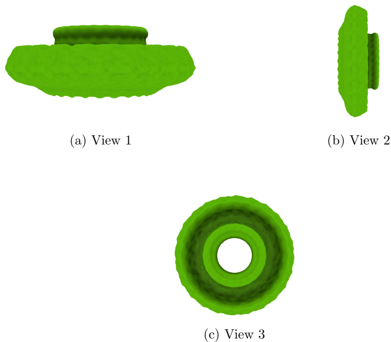
Figure 4: Isosurface at threshold=0.253000. Views generated by ChimeraX at a the following X, Y, Z angles: View 1 (0, -90, -90), View 2 (-90, 0, -90), View 3 (0, 0, 0).
