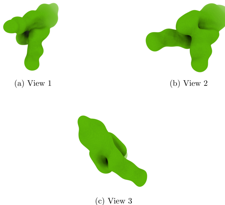
Figure 4: Isosurface at threshold=2.490000. Views generated by ChimeraX at a the following X, Y, Z angles: View 1 (0, -90, -90), View 2 (-90, 0, -90), View 3 (0, 0, 0).
