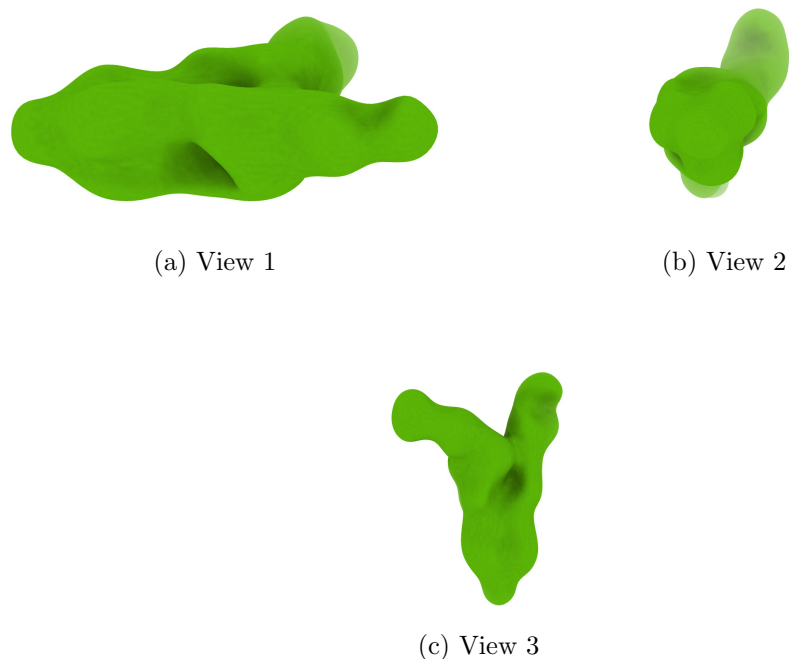
Figure 4: Isosurface at threshold=2.490000. Views generated by ChimeraX at a the following X, Y, Z angles: View 1 (0, -90, -90), View 2 (-90, 0, -90), View 3 (0, 0, 0).
