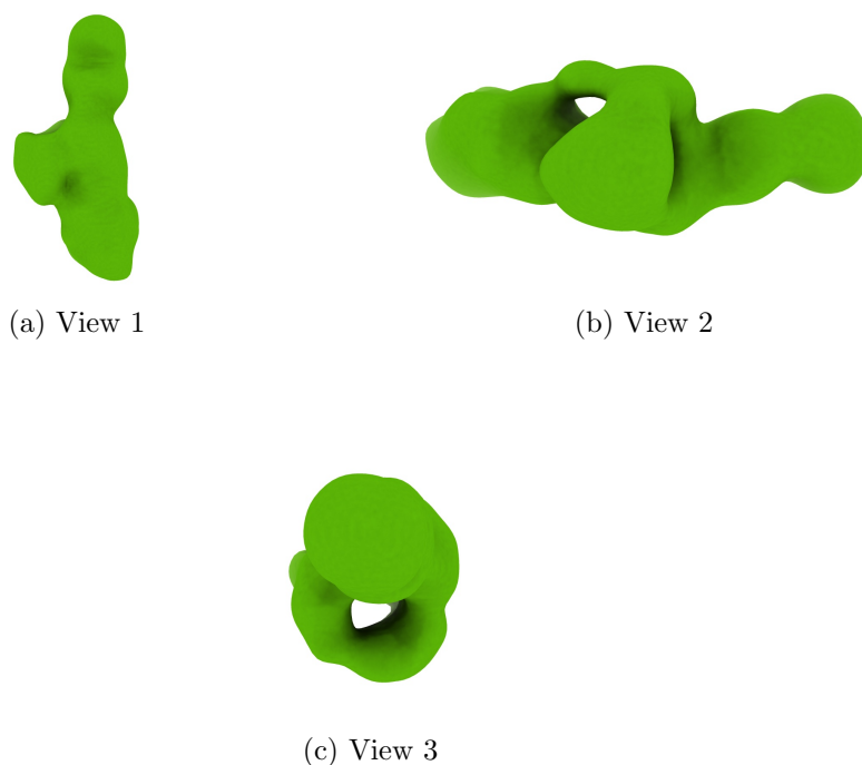
Figure 4: Isosurface at threshold=2.250000. Views generated by ChimeraX at a the following X, Y, Z angles: View 1 (0, -90, -90), View 2 (-90, 0, -90), View 3 (0, 0, 0).
