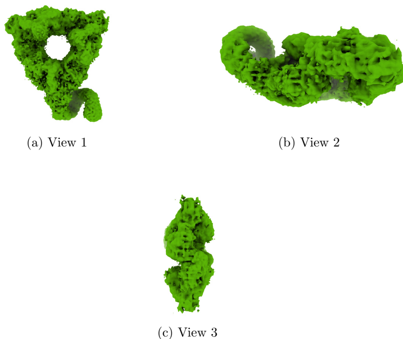
Figure 4: Isosurface at threshold=0.290000. Views generated by ChimeraX at a the following X, Y, Z angles: View 1 (0, -90, -90), View 2 (-90, 0, -90), View 3 (0, 0, 0).
