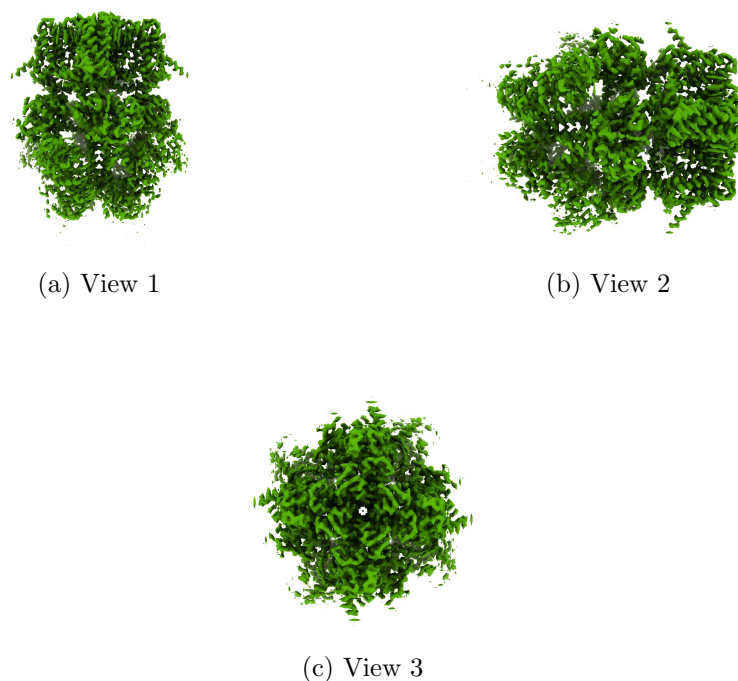
Figure 4: Isosurface at threshold=0.225000. Views generated by ChimeraX at a the following X, Y, Z angles: View 1 (0, -90, -90), View 2 (-90, 0, -90), View 3 (0, 0, 0).
