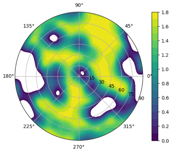
Figure 33: Directional resolution in the projection sphere.
