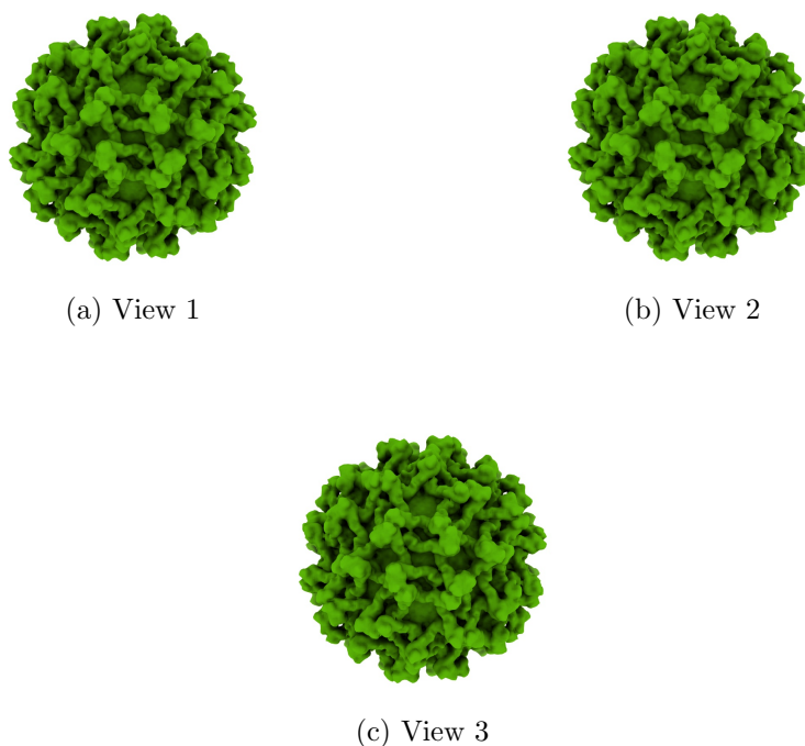
Figure 4: Isosurface at threshold=0.023700. Views generated by ChimeraX at a the following X, Y, Z angles: View 1 (0, -90, -90), View 2 (-90, 0, -90), View 3 (0, 0, 0).
