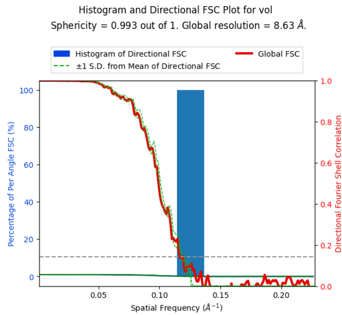
Figure 31: Global FSC and histogram of the directional FSC.
