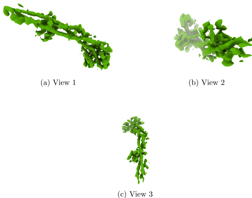
Figure 4: Isosurface at threshold=0.400000. Views generated by ChimeraX at a the following X, Y, Z angles: View 1 (0, -90, -90), View 2 (-90, 0, -90), View 3 (0, 0, 0).
