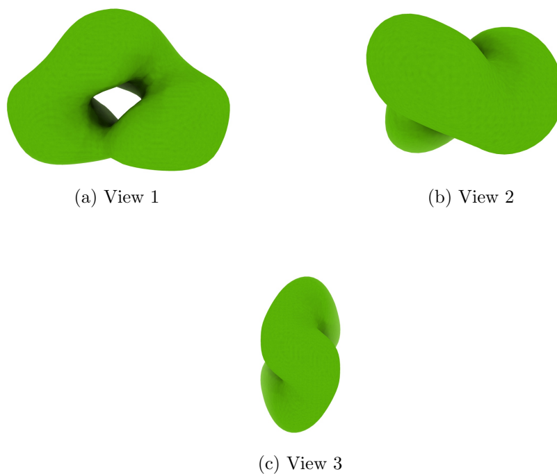
Figure 4: Isosurface at threshold=8.600000. Views generated by ChimeraX at a the following X, Y, Z angles: View 1 (0, -90, -90), View 2 (-90, 0, -90), View 3 (0, 0, 0).
