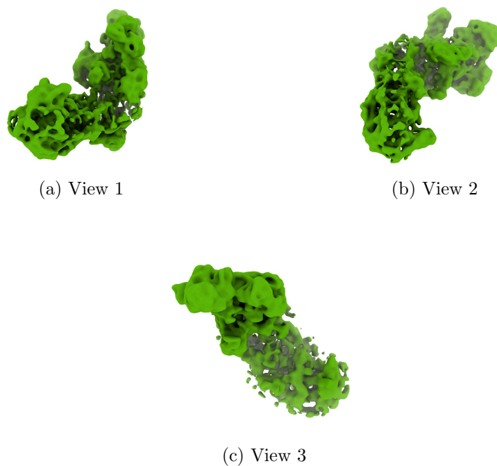
Figure 4: Isosurface at threshold=0.090200. Views generated by ChimeraX at a the following X, Y, Z angles: View 1 (0, -90, -90), View 2 (-90, 0, -90), View 3 (0, 0, 0).
