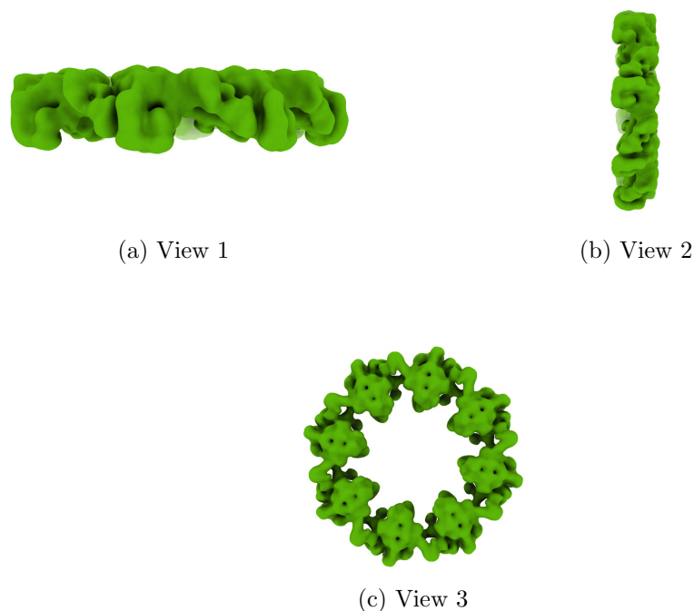
Figure 4: Isosurface at threshold=0.006100. Views generated by ChimeraX at a the following X, Y, Z angles: View 1 (0, -90, -90), View 2 (-90, 0, -90), View 3 (0, 0, 0).
