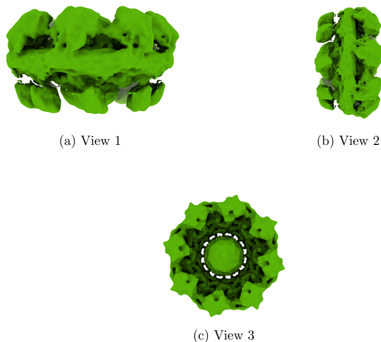
Figure 4: Isosurface at threshold=0.008600. Views generated by ChimeraX at a the following X, Y, Z angles: View 1 (0, -90, -90), View 2 (-90, 0, -90), View 3 (0, 0, 0).
