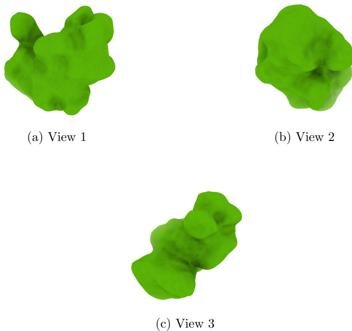
Figure 4: Isosurface at threshold=0.000137. Views generated by ChimeraX at a the following X, Y, Z angles: View 1 (0, -90, -90), View 2 (-90, 0, -90), View 3 (0, 0, 0).
