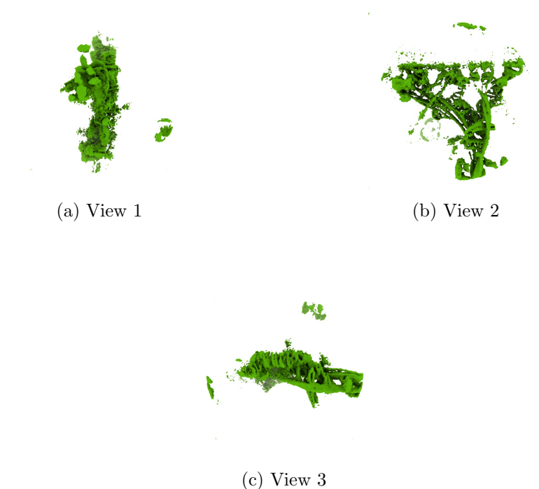
Figure 4: Isosurface at threshold=0.032900. Views generated by ChimeraX at a the following X, Y, Z angles: View 1 (0, -90, -90), View 2 (-90, 0, -90), View 3 (0, 0, 0).
