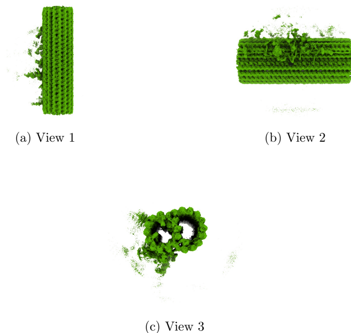
Figure 4: Isosurface at threshold=0.819000. Views generated by ChimeraX at a the following X, Y, Z angles: View 1 (0, -90, -90), View 2 (-90, 0, -90), View 3 (0, 0, 0).
