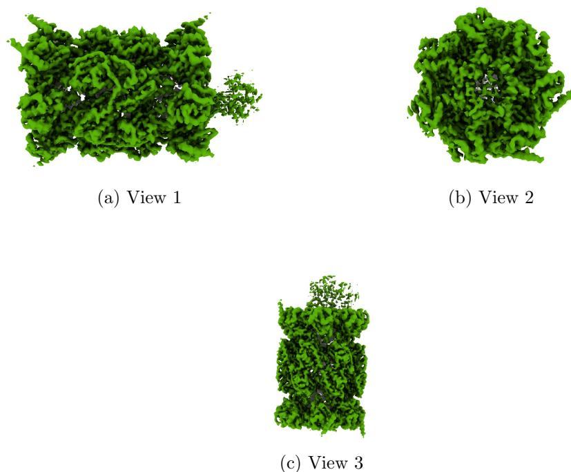
Figure 4: Isosurface at threshold=6.000000. Views generated by ChimeraX at a the following X, Y, Z angles: View 1 (0, -90, -90), View 2 (-90, 0, -90), View 3 (0, 0, 0).
