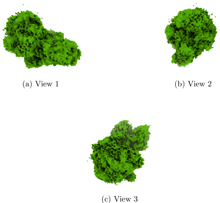
Figure 4: Isosurface at threshold=0.047700. Views generated by ChimeraX at a the following X, Y, Z angles: View 1 (0, -90, -90), View 2 (-90, 0, -90), View 3 (0, 0, 0).
